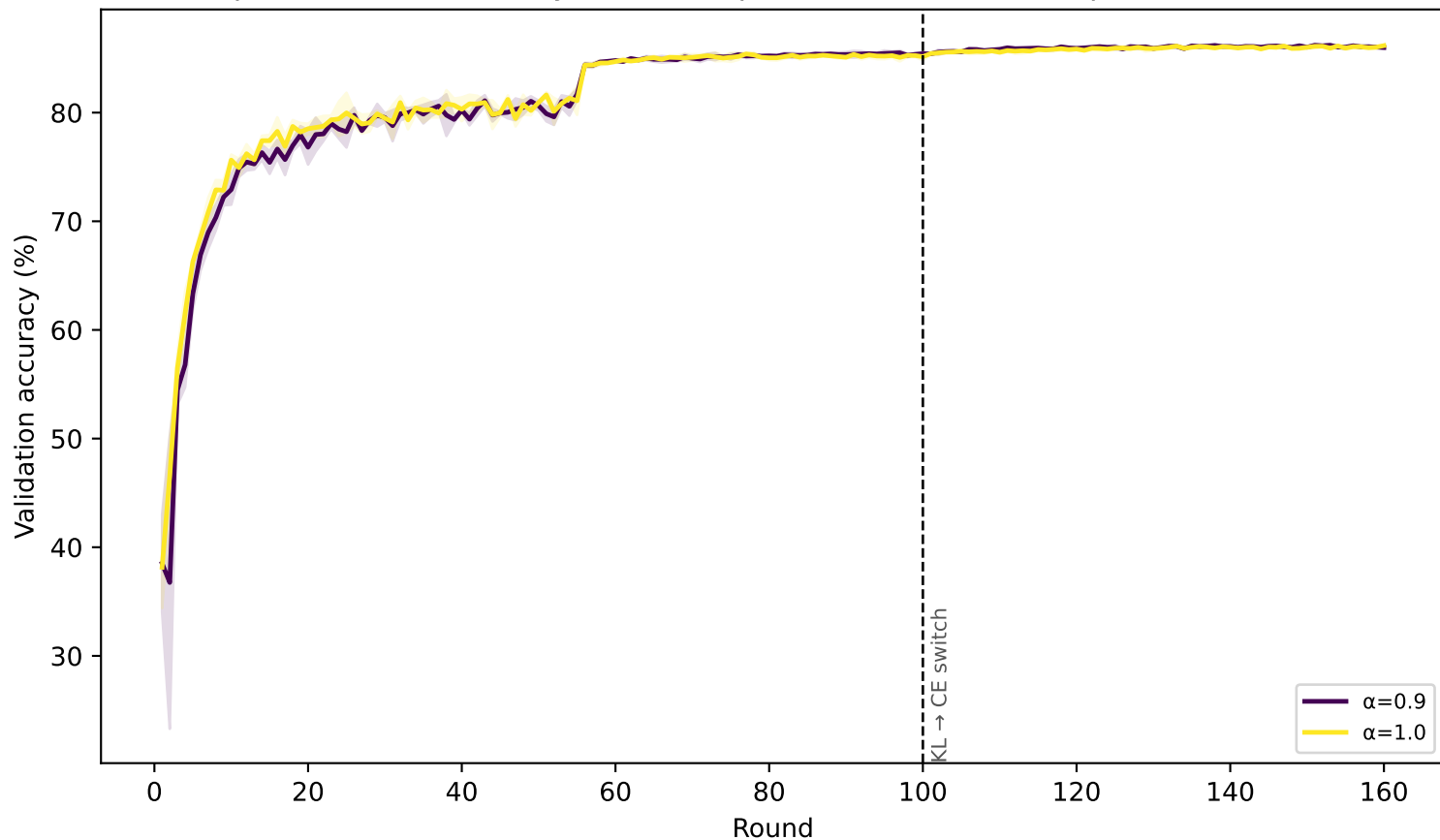
Exp 1: student accuracy across KL phase (1-100) and CE phase (101-160)
